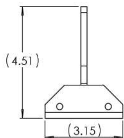
FRONT MOUNT BRACKETS x2
