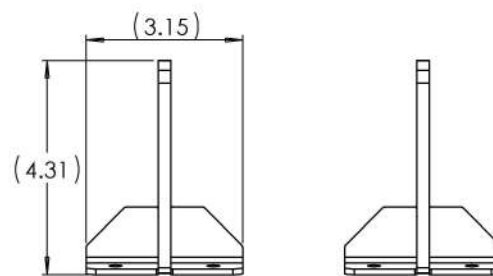
FRONT MOUNT BRACKET x2
