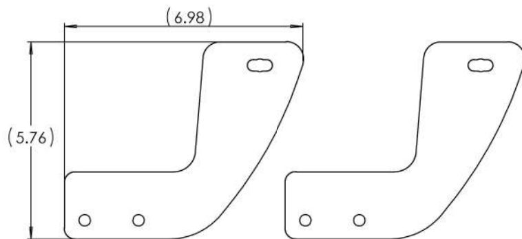
REAR MOUNT BRACKETS x2
